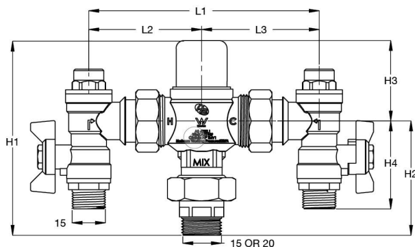
Figure 1 – Physical Size CLINIMIX ® TMV – NICKEL PLATED FINISH with 1/2" Male Thread Inlet and Outlet Fittings.
